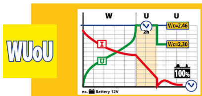
Integrated charger 230V ≈ 50/60 Hz Charging current: 7A average / 11A efficient
