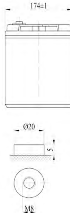
Battery Dimension terminal size
